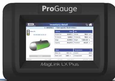
ProGauge MagLink LX Plus console
